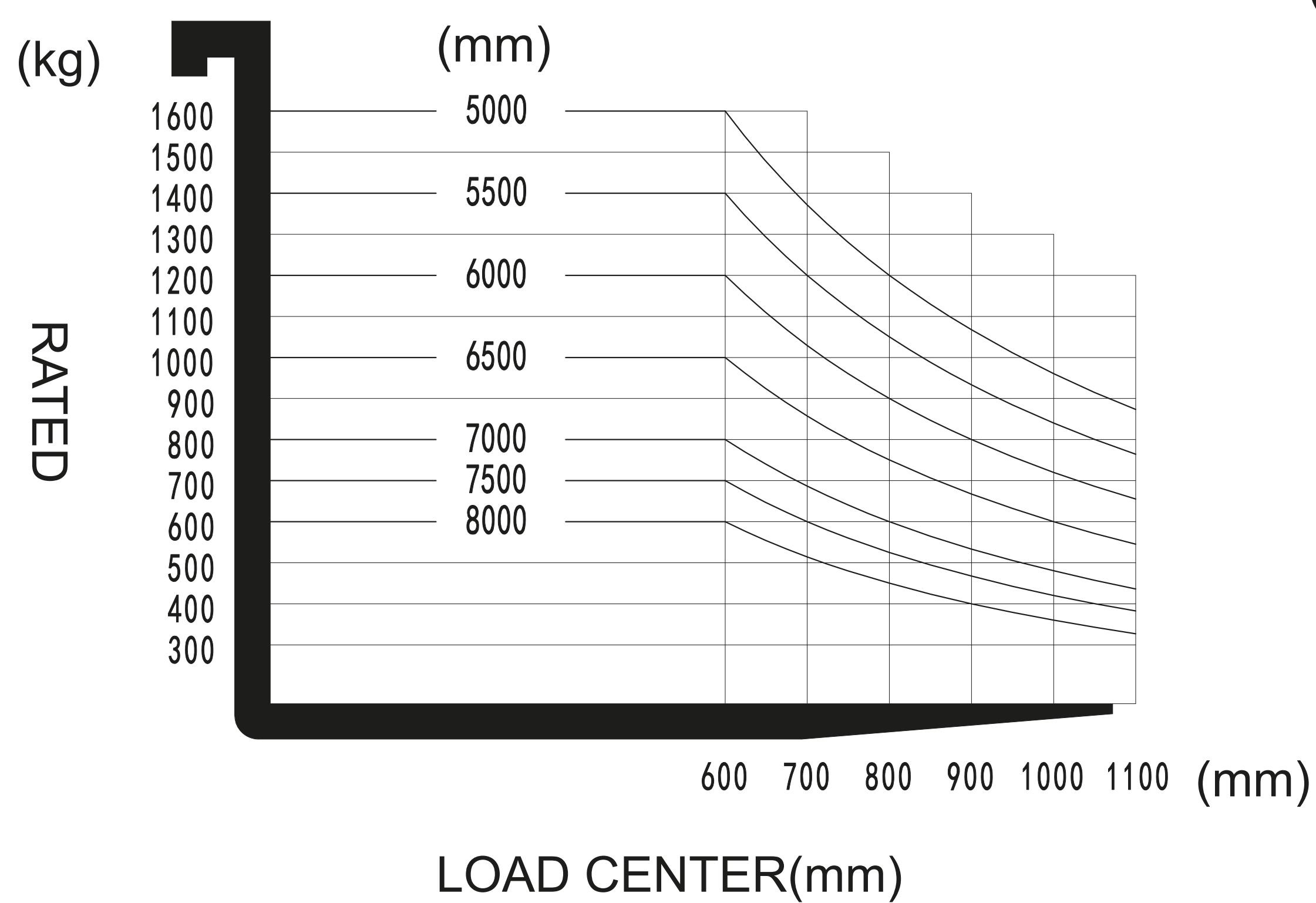
RATED CAPACITIES GRAPH
