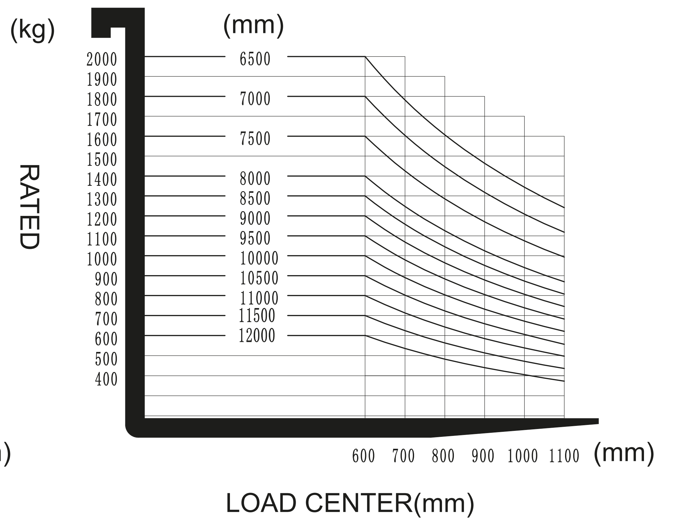
RATED CAPACITIES GRAPH
